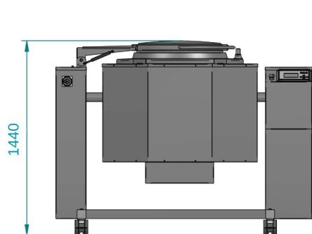
VISTA FRONTAL
