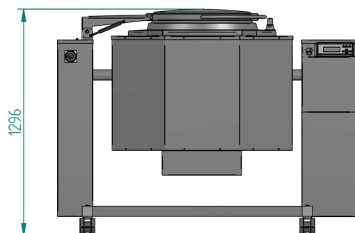
VISTA FRONTAL
