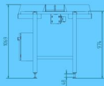
VISTA FRONTAL
